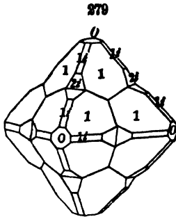
Chalcopyrite.
